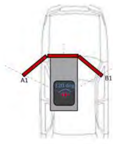
Figure 2: Representation of a compressed visual system displaying 180 degrees of graphic information in an optical (physical) FOV of 120 degrees
