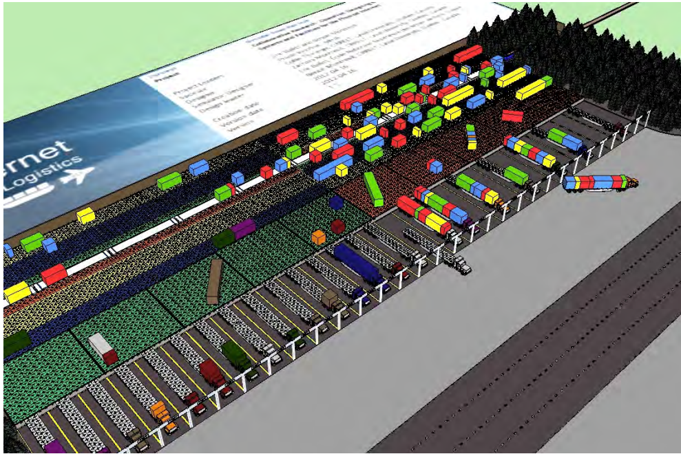
Figure 12: Final Layout Focusing on Rail Operations of the Proposed Design
